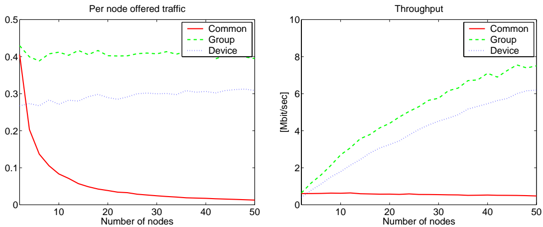
Figure 13: Per node offered traffic and total throughput as the number of groups are increased. Group size is fixed at 2.
